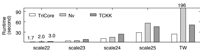
Fig. 11: TRICORE vs Graph Challenge champions. Note, similarly to Nv, the time of TRICORE is on one Titan X GPU.
