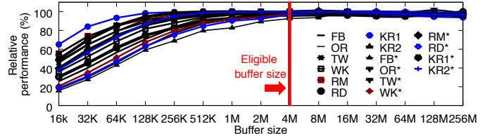
Fig. 8: Relative performance with respect to various buffer sizes. The legend with ‘*’ means the result is on Titan X, otherwise it is on K40c. For example, TW and TW* mean the results of TW on K40c and Titan X, respectively.
