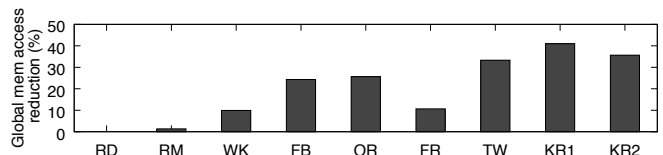
Fig. 6: Percentage of GPU global memory access transactions reduced by shared memory optimization.
