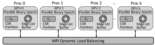
Fig. 3: TRICORE framework.
