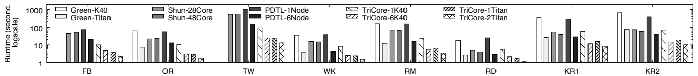
Fig. 10: The runtime of TRICORE and three related projects: Green [27] (on single K40c and single Titan X GPU), Shun [51] (on 28-core CPU and 48-core CPU) and PDTL [24] (on single node and 6 nodes of 16-core CPU). TRICORE-1K and TRICORE-6K are our results on one and six K40c GPUs respectively. Similarly, TRICORE-1Titan X and TRICORE-2Titan X are our results on one and two Titan X GPUs respectively. All these GPU results are on a single machine.
